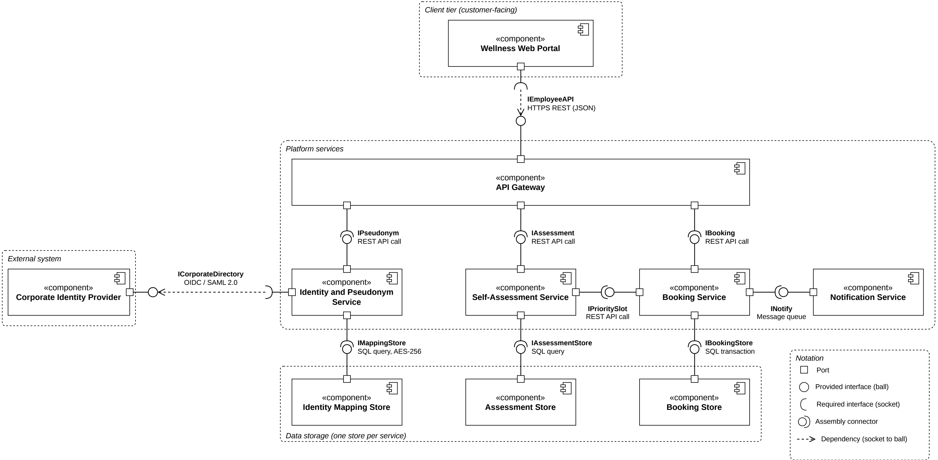
UML Component Diagram: Corporate Mental Wellness and Counseling Platform (Microservices)
